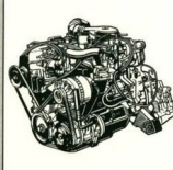
2.6-liter (155.9 CID) four-cylinder balance shaft engine: 104 hp @ 4,800 rpm; 142 lb-ft torque @ 2,800 rpm.†
