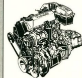
Turbocharged 2.2-liter (135 CID) four-cylinder electronically fuel injected engine: 146 hp @ 5,200 rpm; 170 lb-ft torque @ 3,600 rpm.†
