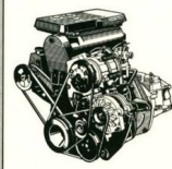
2.5-liter four-cylinder electronically fuel injected balance shaft engine: 100 hp @ 4,800 rpm; 136 lb-ft torque @ 2,800 rpm.
