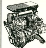
2.2-liter (135 CID) four-cylinder electronically fuel injected engine: 97 hp @ 5,200 rpm; 122 lb-ft torque @ 3,200 rpm.
