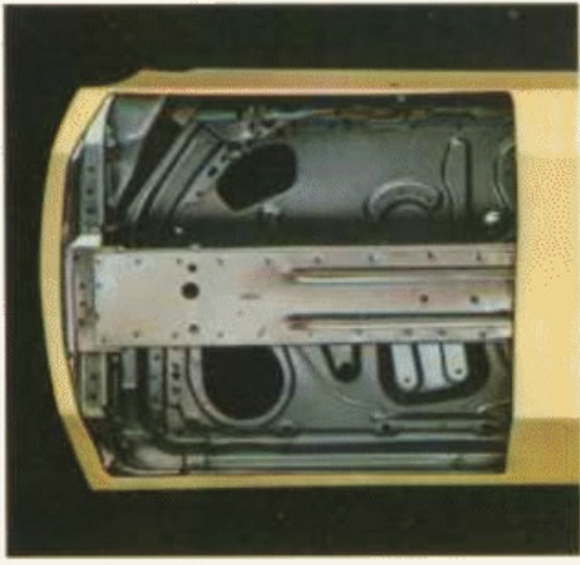
Side-door guard beam.
