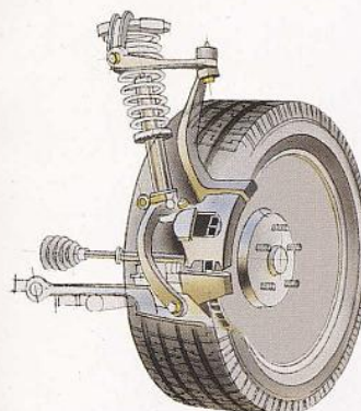
Power-assisted front disc brakes.
