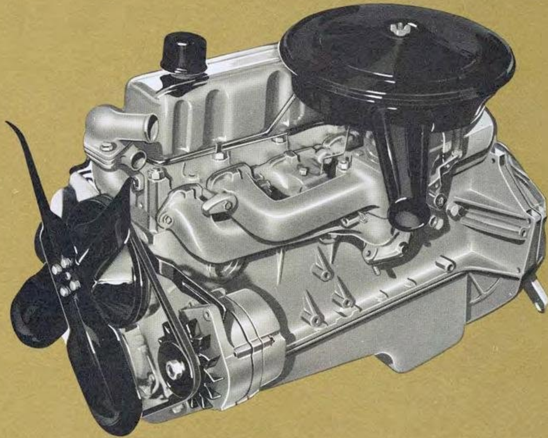
HI-THRIFT 194 ENGINE
