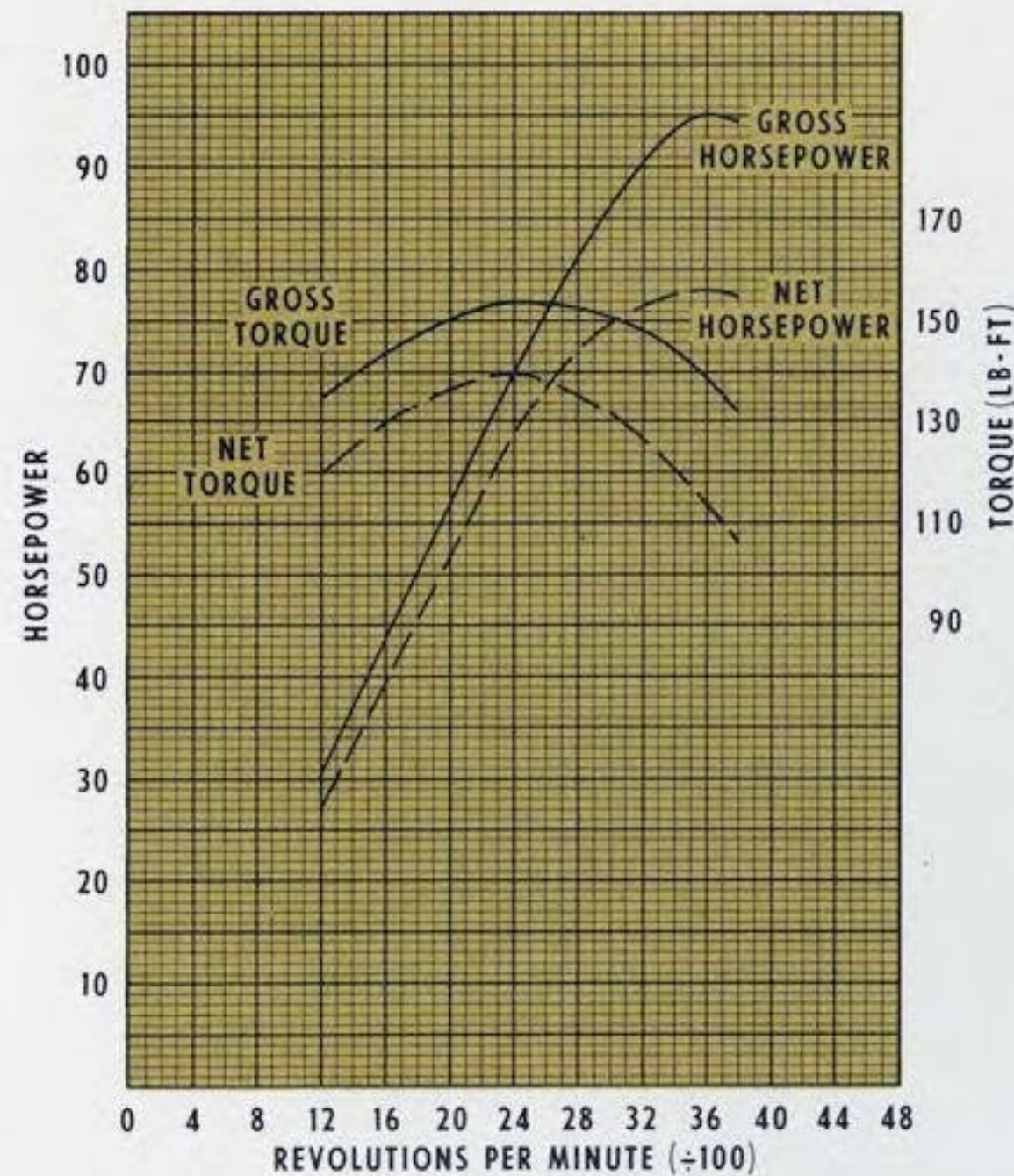
WITH REGULAR CAMSHAFT
