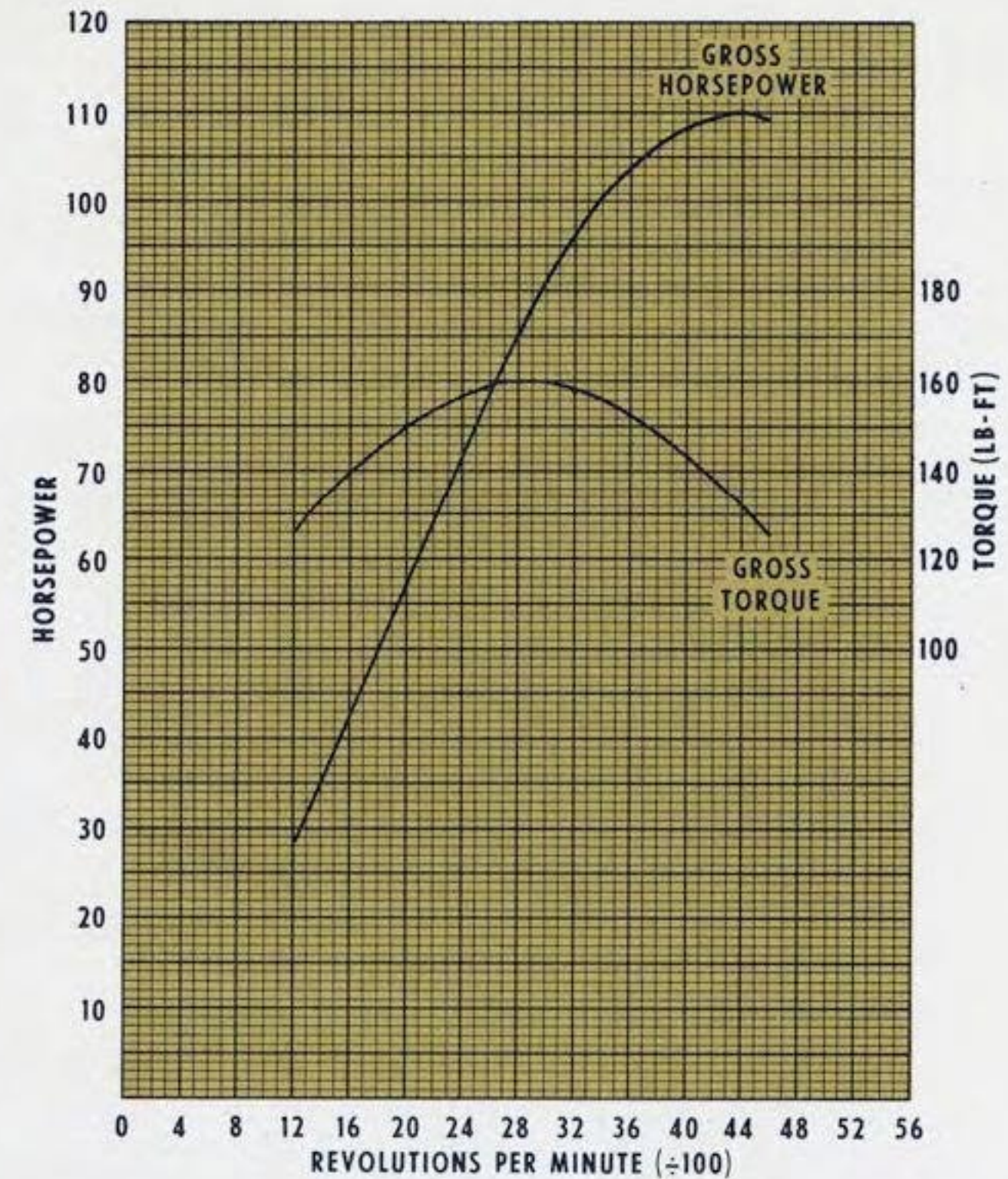
WITH SPECIAL CAMSHAFT
