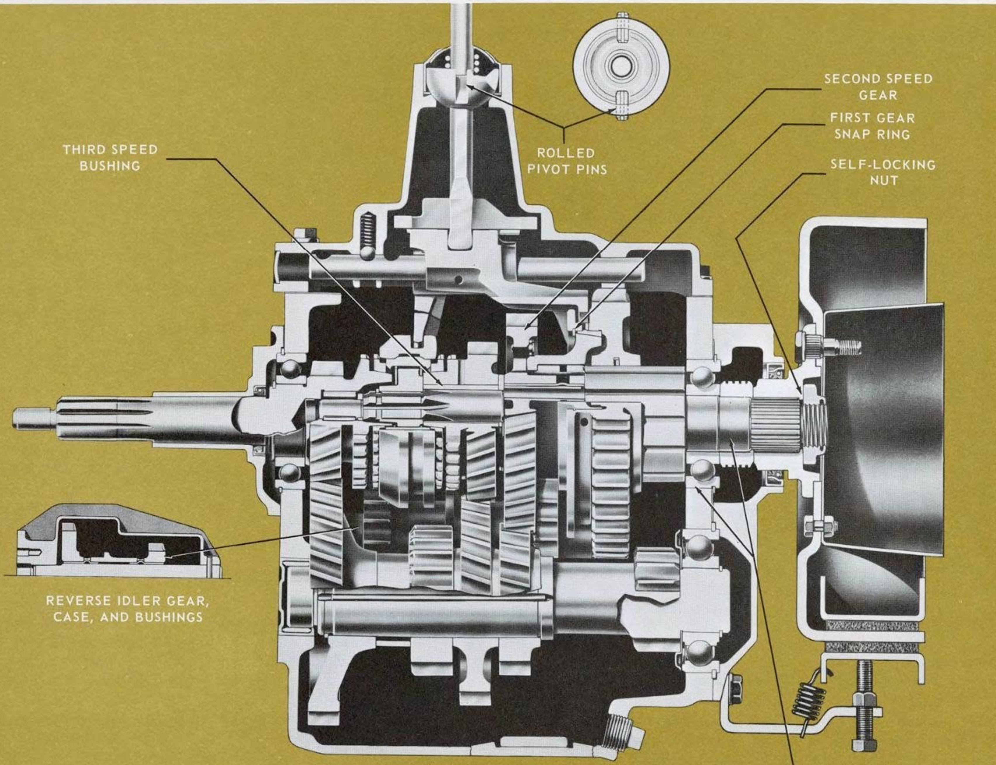
IMPROVED 4-SPEED TRANSMISSION
