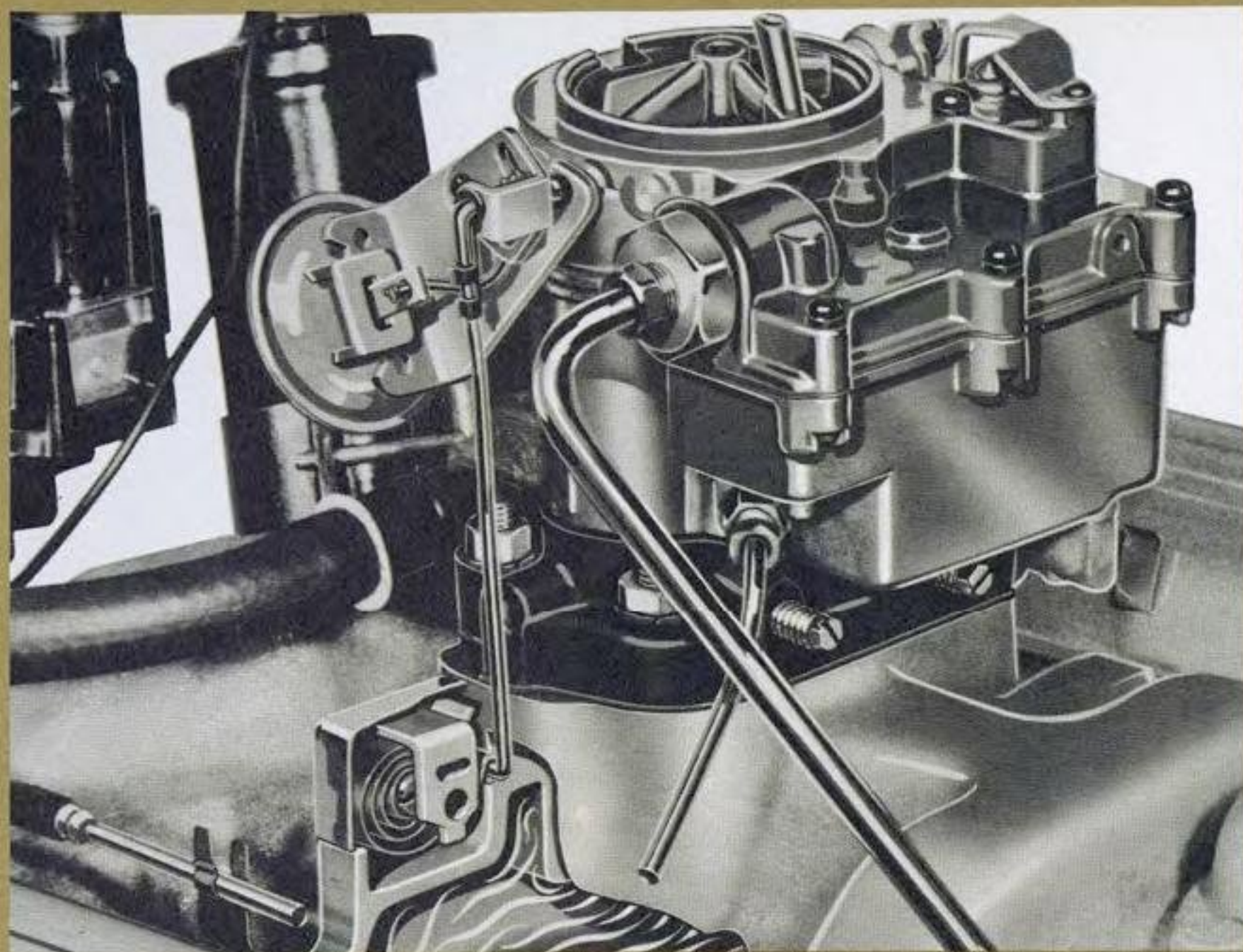
V-8 AUTOMATIC CHOKE CONTROL
