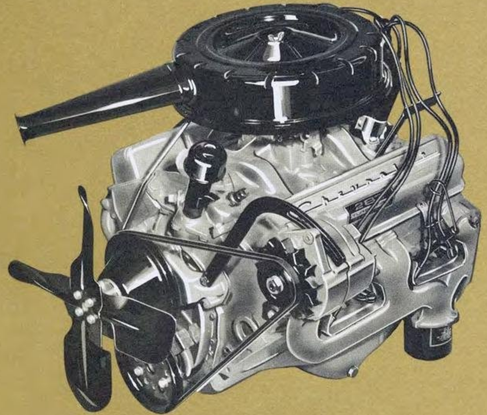
TURBO-FIRE 283 ENGINE
