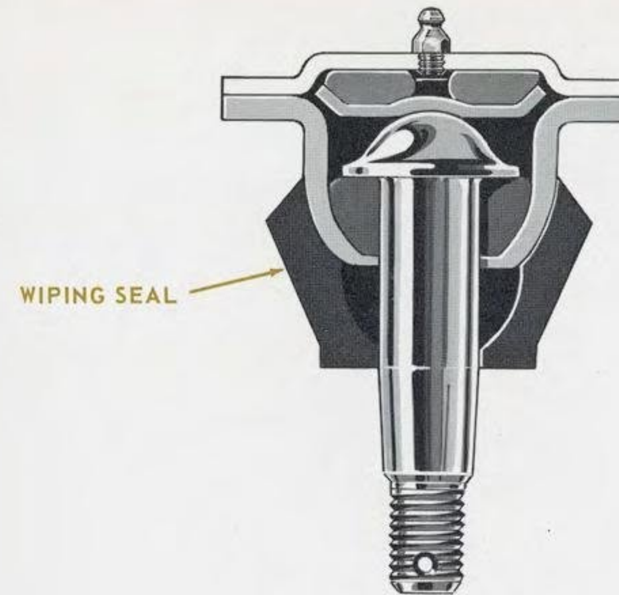
1963 SPHERICAL JOINT
