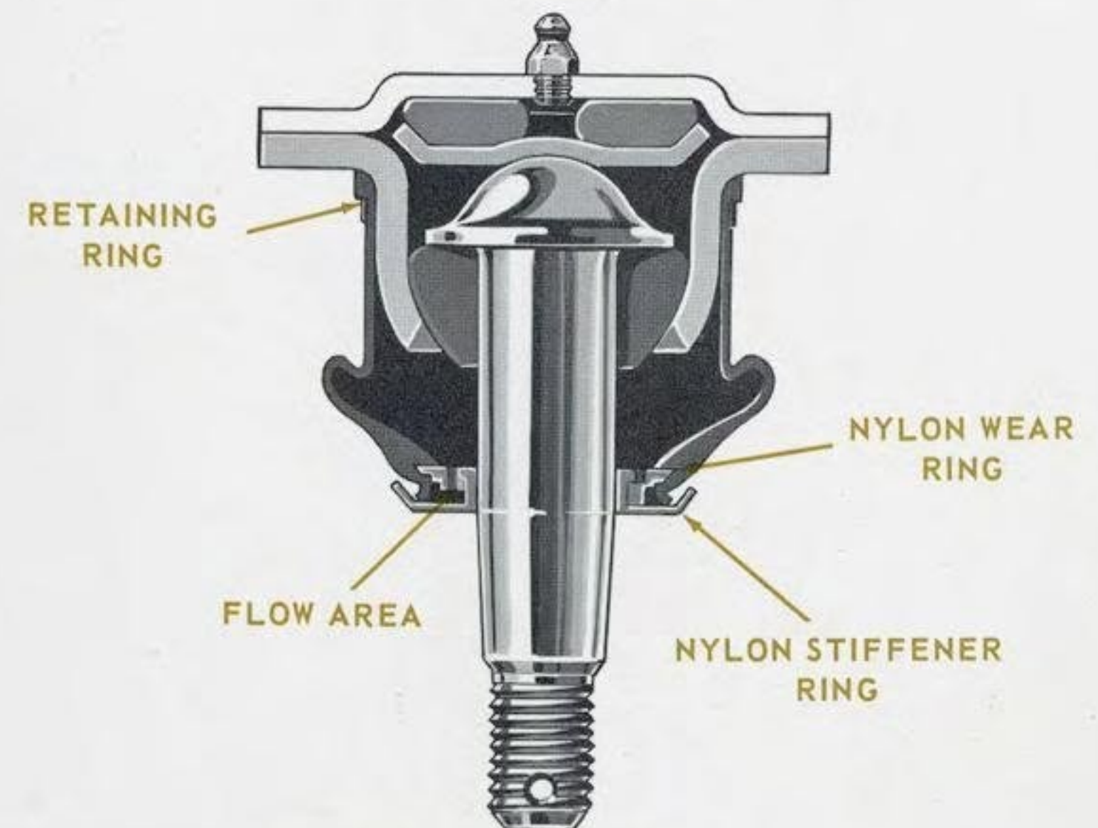
1964 SPHERICAL JOINT
