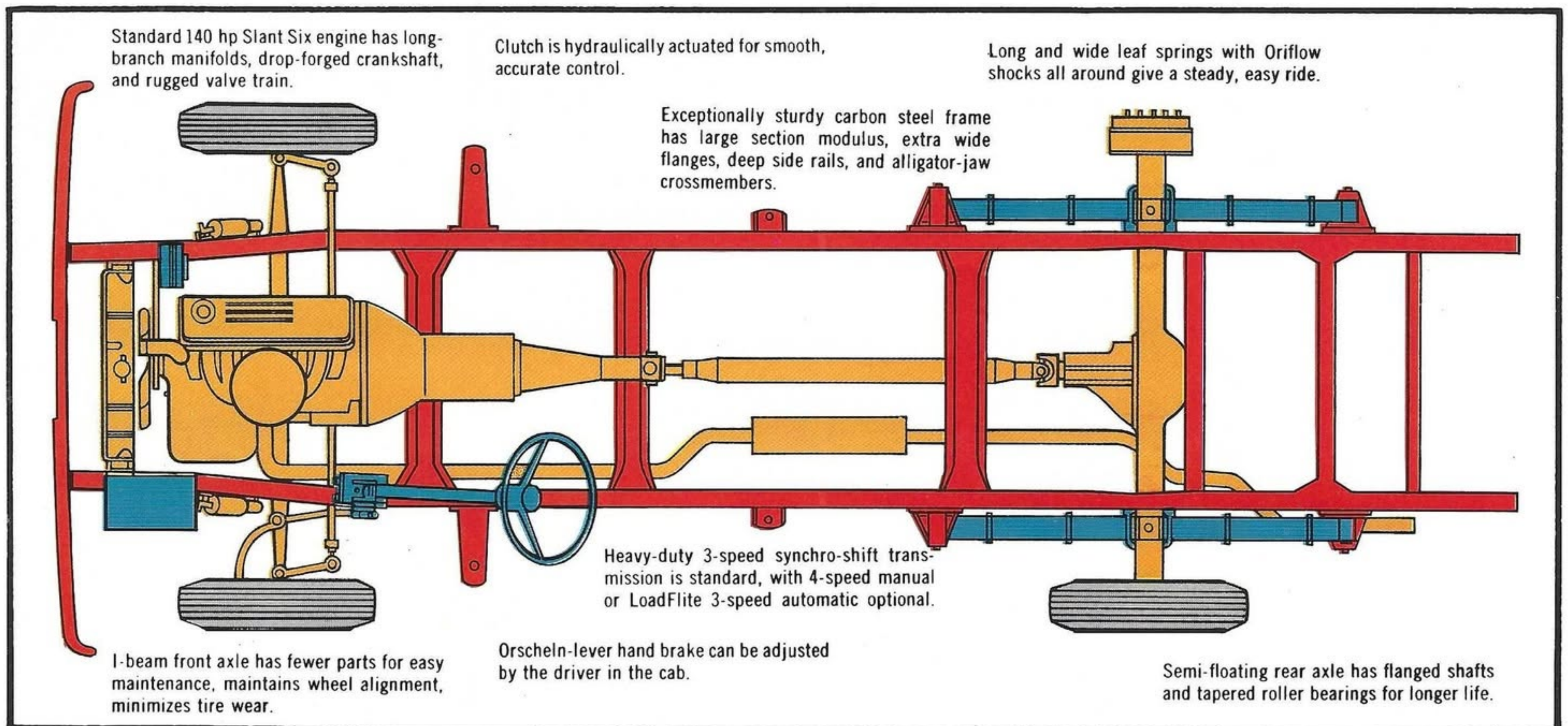
D100 Town Panel and Town Wagon on 114" wheelbase.
