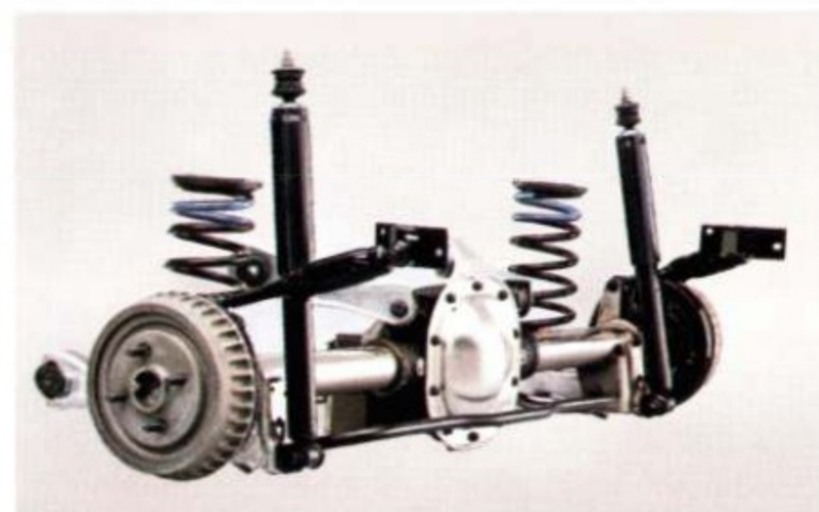
Rear Quadra-shock suspension of GT (also included with the 5.0L EFI HO engine option) consists of vertically-mounted, gas-pressurized shocks, horizontally-mounted axle dampers and a stabilizer bar. The coil springs are the progressive rate-type and range from 200-300 lb./in.
