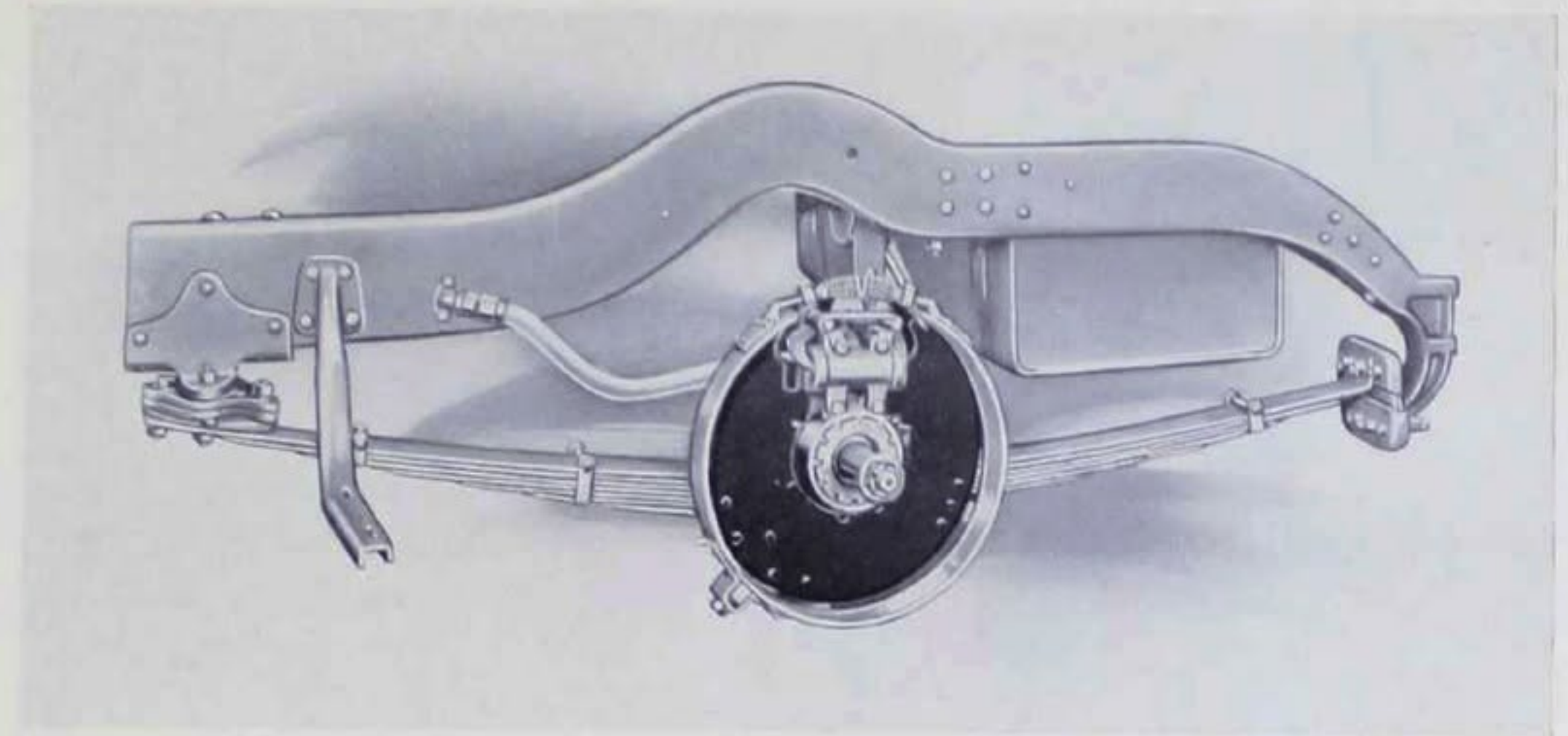
FABRIC SHACKLE CONSTRUCTION [Rear End]
