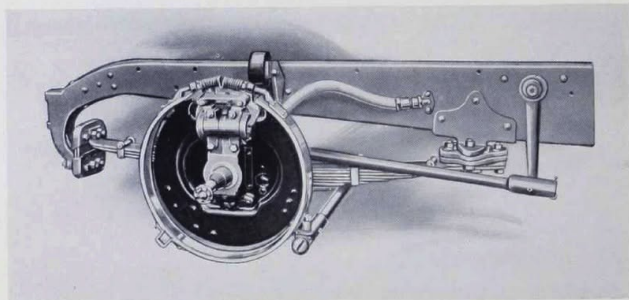
FABRIC SHACKLE CONSTRUCTION [Front End]
